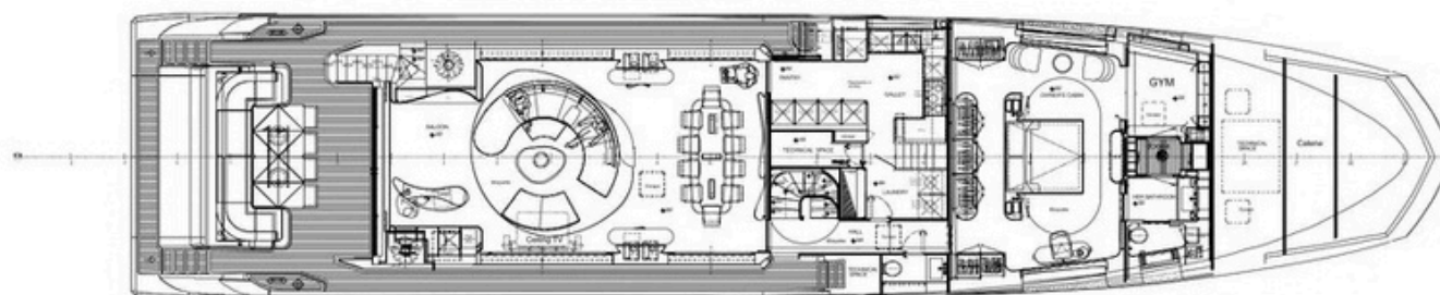
Main deck
