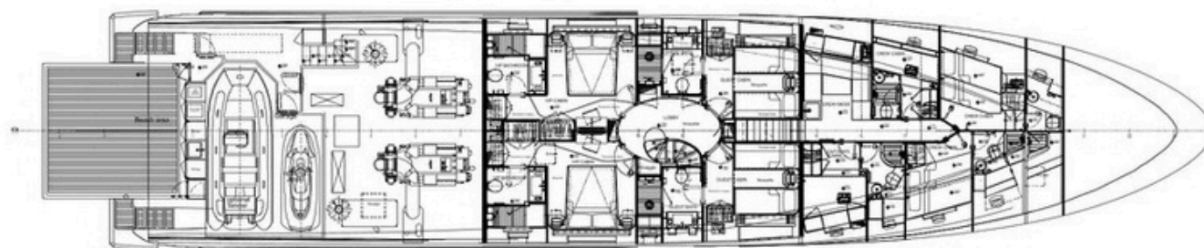
Lower deck
